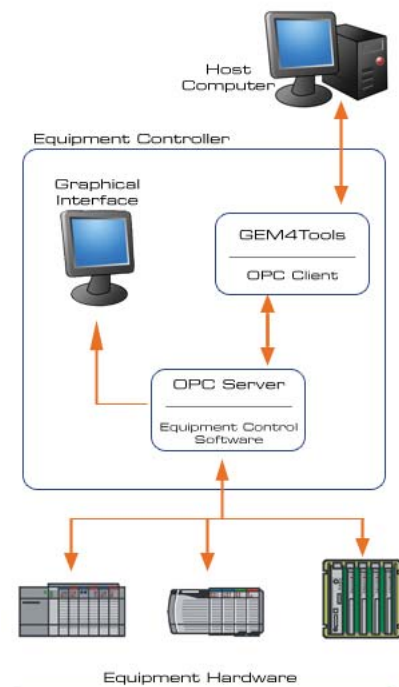
System Architecture
